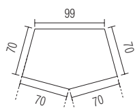
Trapeziform worktop
