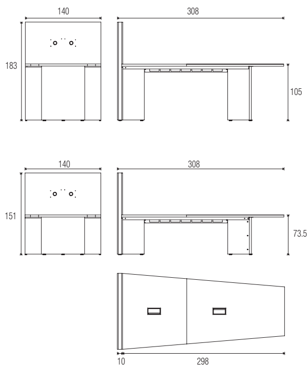
Trapeziform worktops
