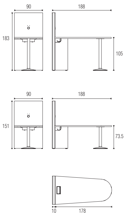
Curved worktops
